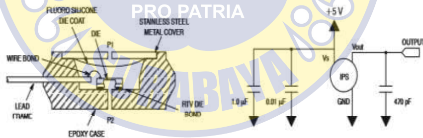
Figure 3. Cross-Sectional Diagram (Not to Scale)
