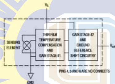
Figure 1. Fully Integrated Pressure Sensor Schematic
