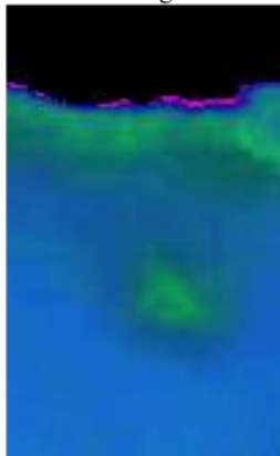
Gambar 7. HSV model
