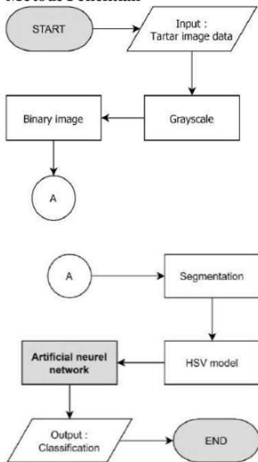
Gambar 1. Flowchart Sistem
