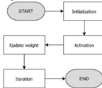
Gambar 8. Flowchart ANN
