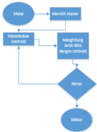
Gambar 1. Alur K-Means
