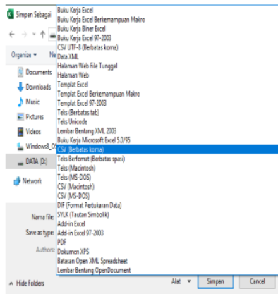
Gambar 4. Proses Delimiter
