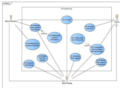
Gambar 2. Diagram Use case
