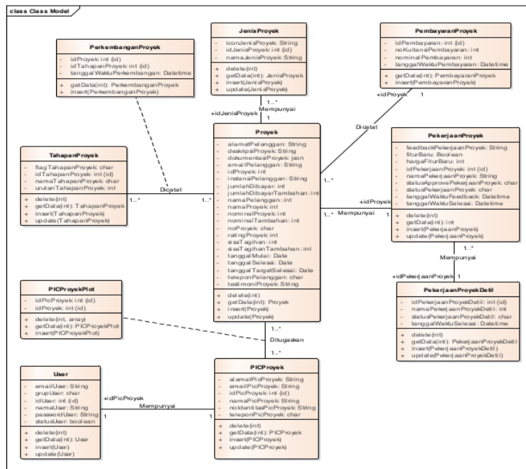
Gambar 3. Class Diagram
