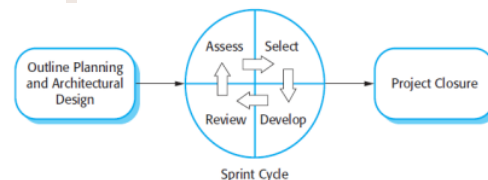
Gambar 1. Proses Scrum [2]
