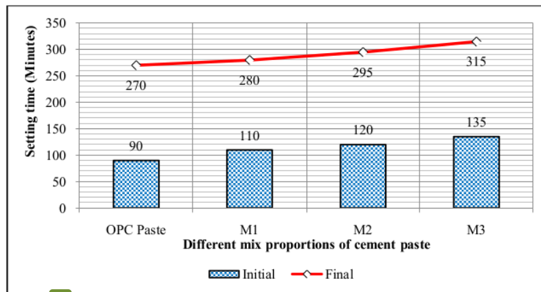
10 Fig. 2: Initial and final setting time of cement paste with and without ground CBA
