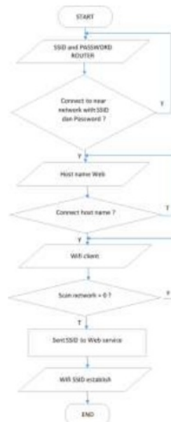
Gambar 5. Flowchart Router
