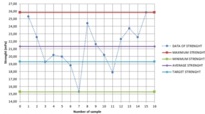
Figure 2. Graph of strength test results with a coarse aggregate of crushed stone.
