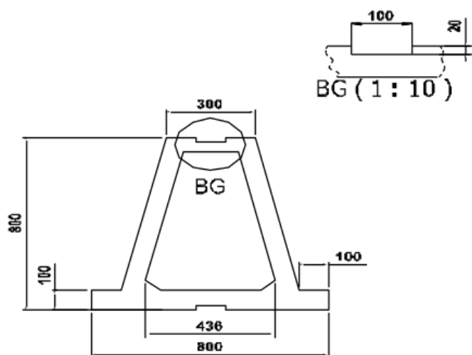
Precast Foundation
