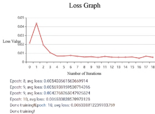
Fig. 6. Loss graph using LSTM
