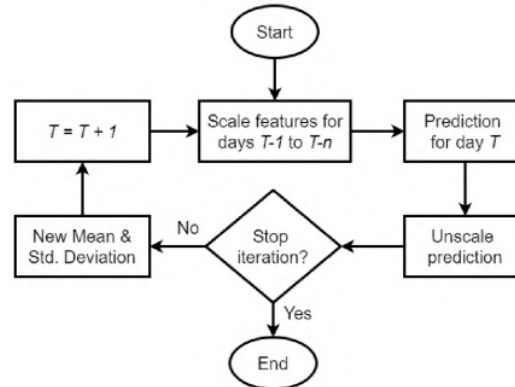
Fig. 2. Logic implementation by recursive forecasting
