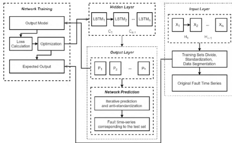
Fig. 3. General LSTM Architecture [17]
