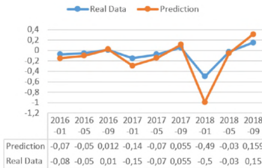
Fig. 4. Plot result shows the predictions using XGBoost
