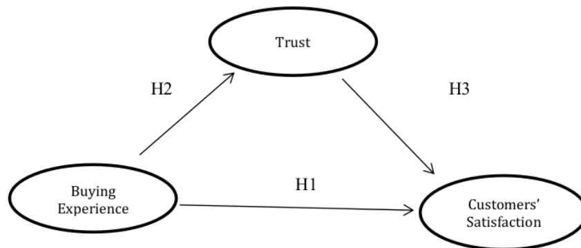
Figure 1. Hypothesis Model
