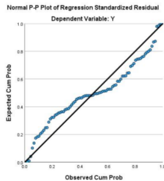
Figure 3. Normality Test Figure
