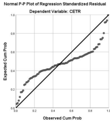
Figure 2. Normality test Figure
