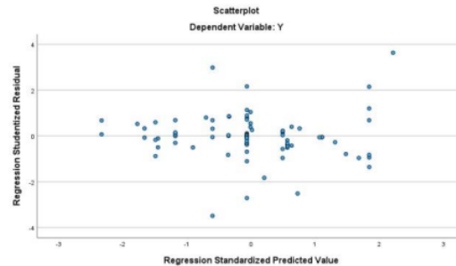
Figure 4. Heteroscedasticity Test Figure Scatterplot
