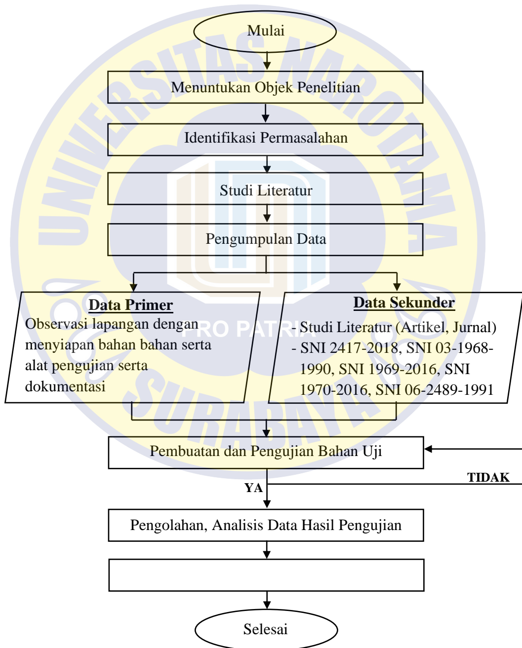
Gambar 3.1 Prosedur Penelitian
