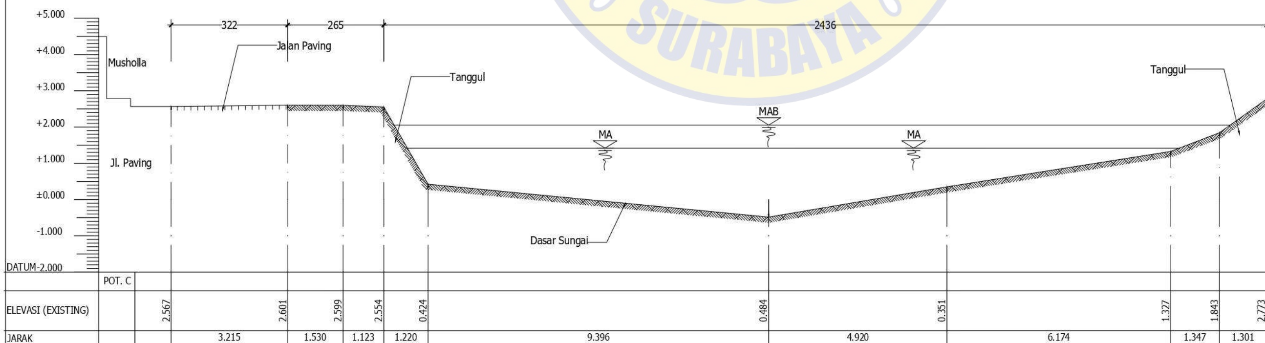
POTONGAN C-C (EXISTING)
