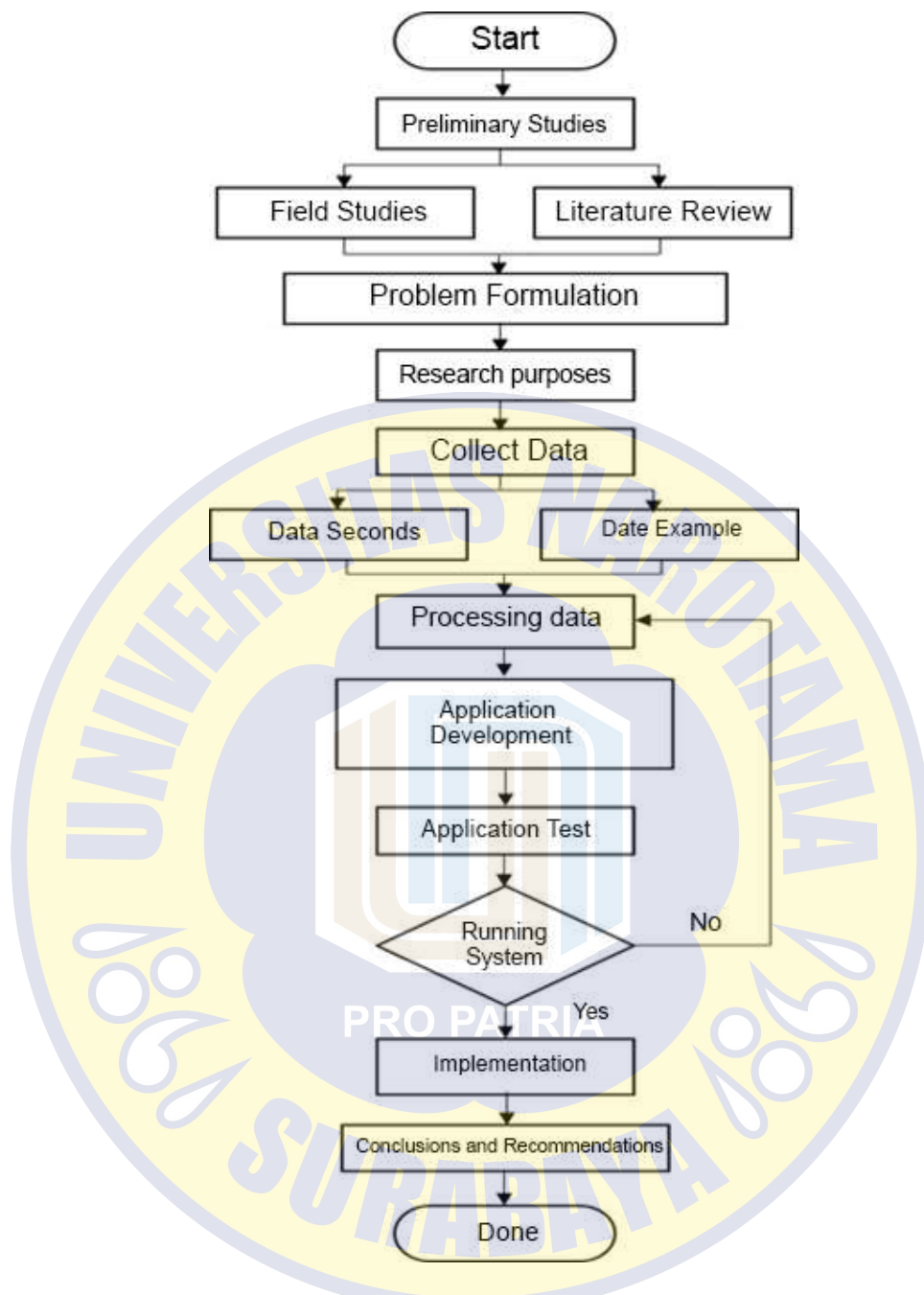
Figure 3.2 Needs Analysis
