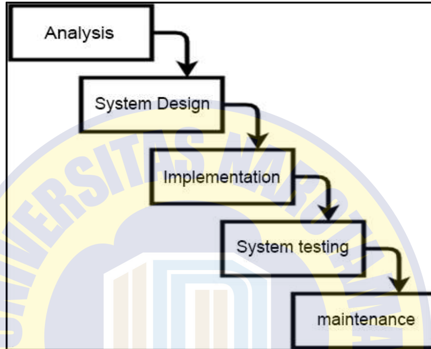
Figure 3.1 Waterfall Model
